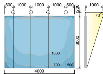
HCF1572BHE + CMT150F/WW 13000 lm
